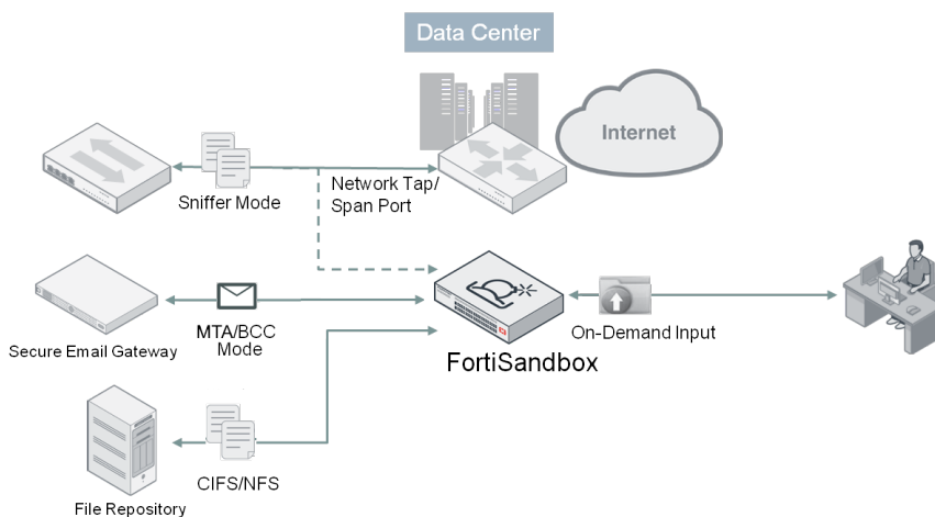
Figure 5 - Standalone deployment
